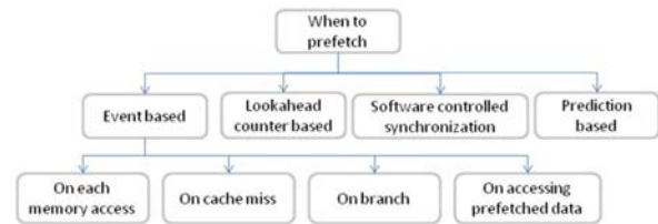
Figure 5. Predicting when to prefetch
