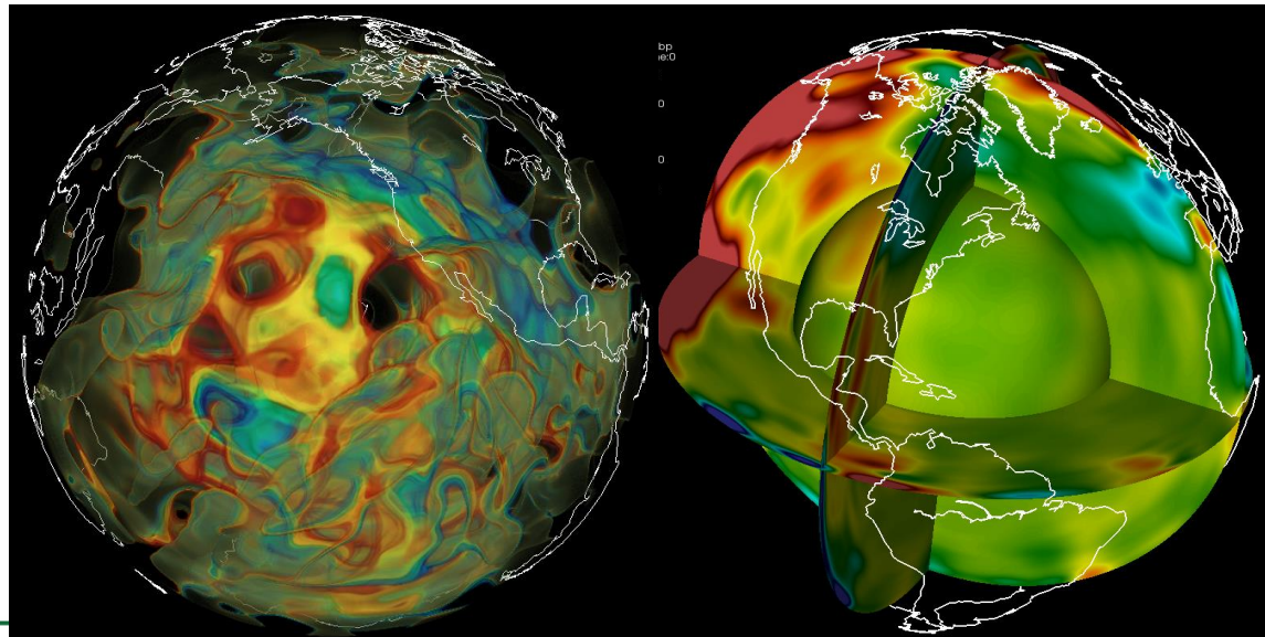
Visualization of data from SpecFM3D. Simulation by J. Tromp (Princeton)
