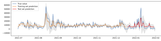
(a) Access counts
