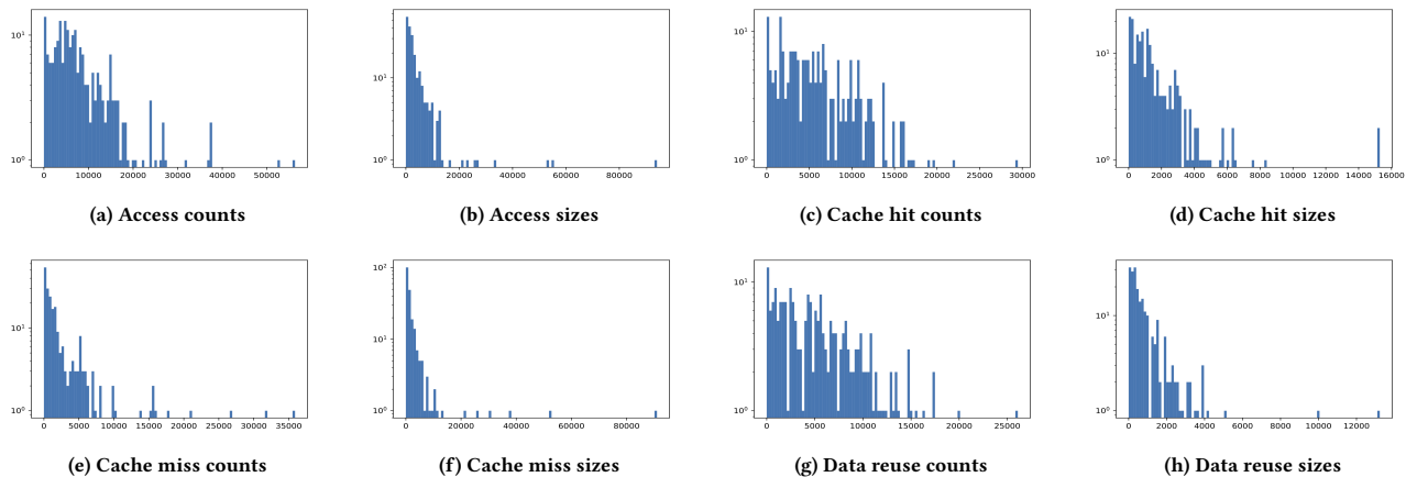
Figure 10: Distribution of daily features
