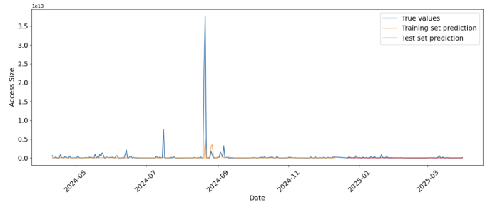
Fig. 9. Daily access size predictions for the 6th most popular dataset, RunIISummer20UL16MiniAODv2/TTToSemiLeptonic_TuneCP5_13TeV-powheg-pythia8, using an LSTM model to predict accesses from April 2024 to April 2025
