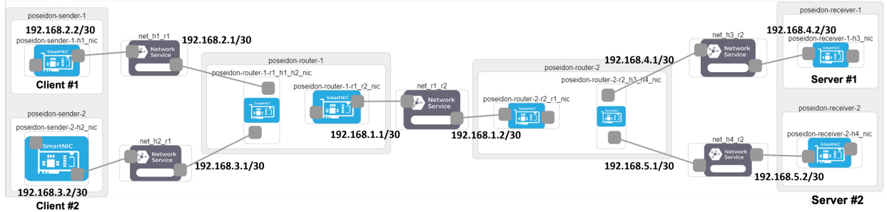
Fig. 3. FABRIC testbed topology mirroring the DISTRI setup. Two senders (Sender #1 and #2) transmit data to two receivers (Receiver #1 and #2) through a network of routers creating a bottleneck, enabling real-world validation of TCP behavior.
