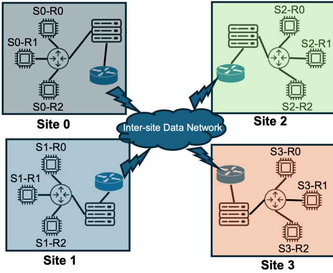
Fig. 2. DISTRI dumbbell topology with four sites. Site 0 and Site 1 host computational resources (S0-R0 and S1-R0) that simultaneously request data from Site 2 and Site 3 DTNs, respectively, creating competing flows through the shared inter-site network.
