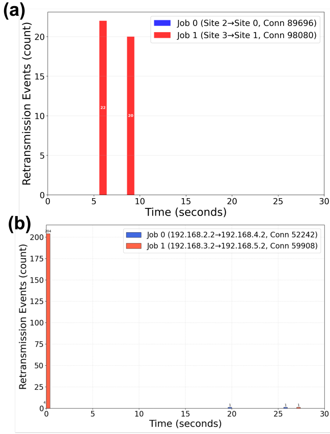
Fig. 5. Retransmission events in DISTRI (a) and FABRIC (b). Job 1 (red) experiences significantly more retransmissions than Job 0 (blue) in both environments. DISTRI shows 22 and 20 retransmission events at 6s and 9s respectively for Job 1, while FABRIC shows 204 early retransmissions for Job 1. This asymmetry directly explains the CWND suppression observed in Fig. 4.
