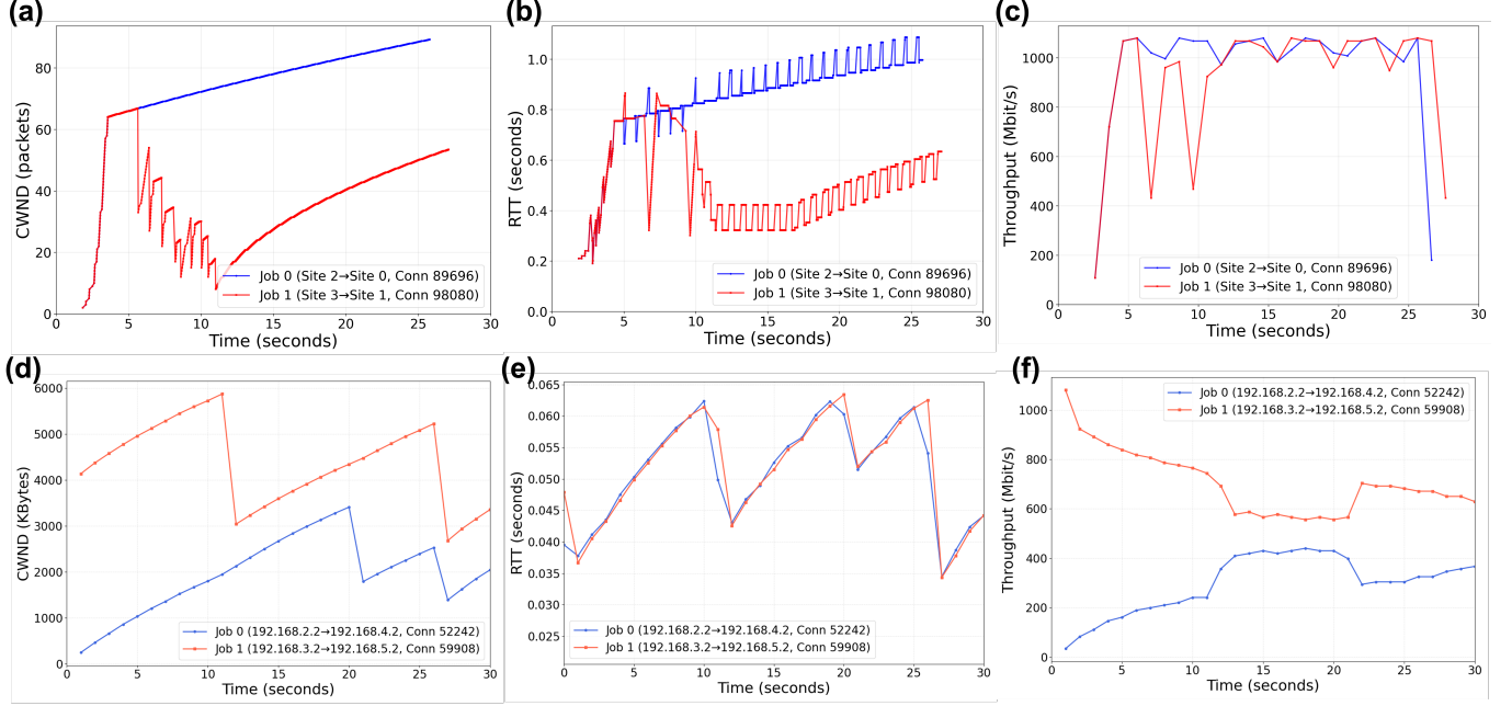
Fig. 4. Comparison of TCP behavior between DISTRI simulation (a-c) and FABRIC testbed (d-f). Top row shows DISTRI results for CWND (a), RTT (b), and throughput (c). Bottom row shows corresponding FABRIC measurements (d-f). Both environments exhibit similar behavioral trends in TCP dynamics despite differences in absolute values.
