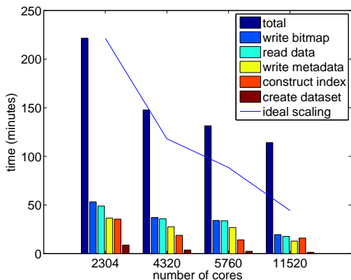
Figure 15: Build index time for 720 time steps (50TB) as the number of cores increases from 2304 to 11,520.
