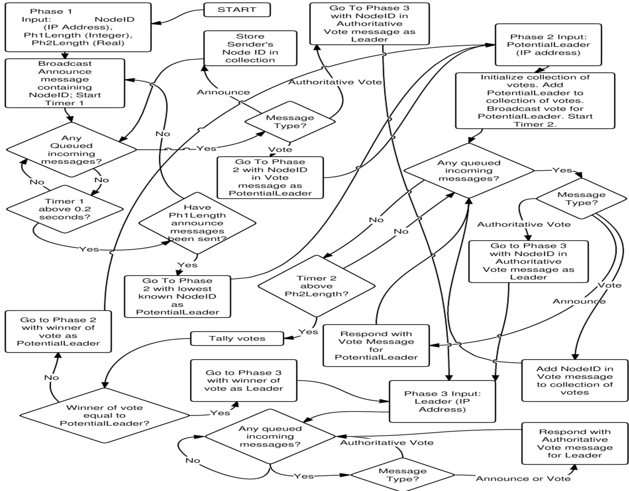
Figure 4: Leader election algorithm
